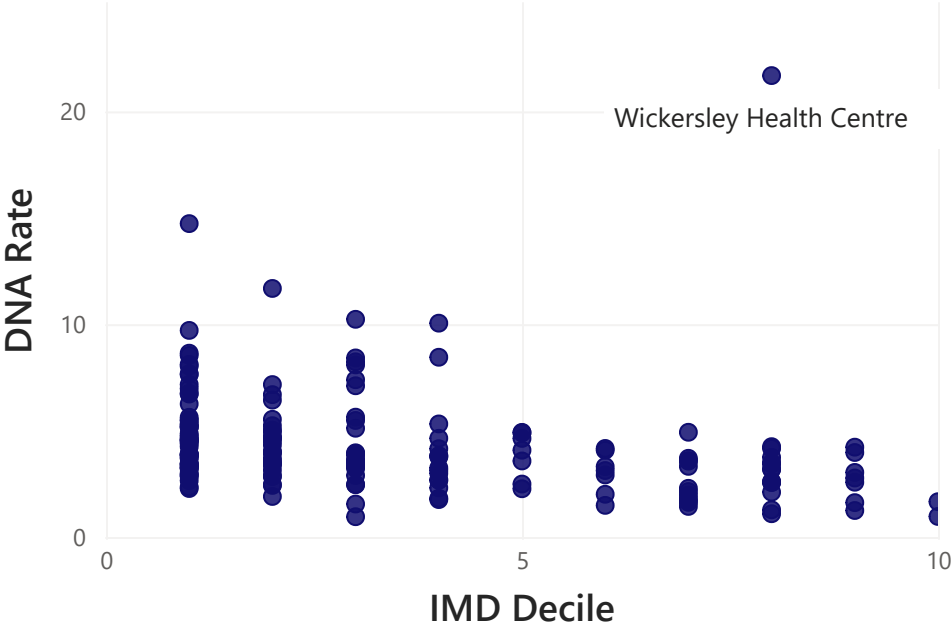
DNA Rate vs Deprivation Decile by Practice
